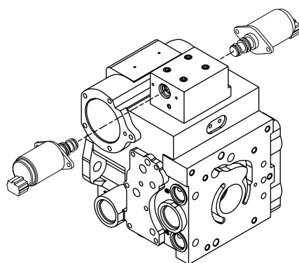
Manifold block NFPE housing
