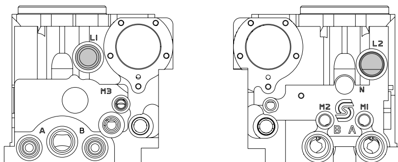
Old Case Drain Locations
