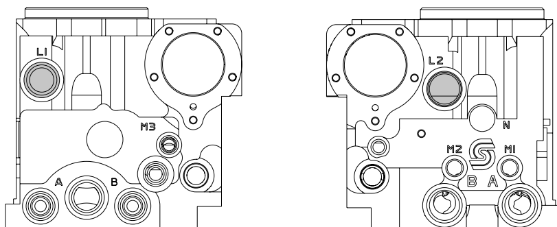
New Case Drain Locations
