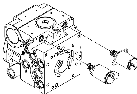
Integral NFPE housing
