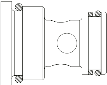
New SCR valve plug
