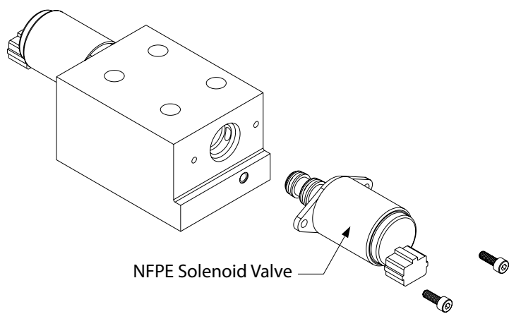
NFPE Control Valve Assembly
