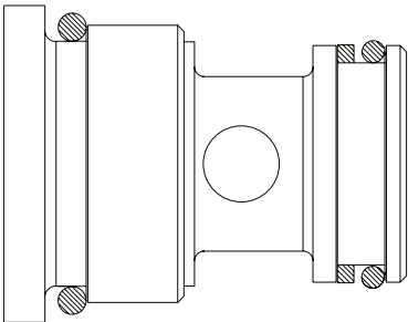
Old SCR valve plug
