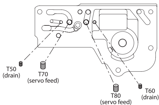
Possible orifice locations
